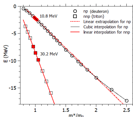
Fig. 1: The ground state energy E of the triton (nnp) (open squares) and deuteron (np) (open circles) as a function of the nucleon mass m^*/m_0 . The black curve corresponds to the cubic fit for the energy-mass dependence, and the red dashed line gives the linear fit for the calculated energies shown by red symbols. The numbers indicated on the averaged kinetic energy.
